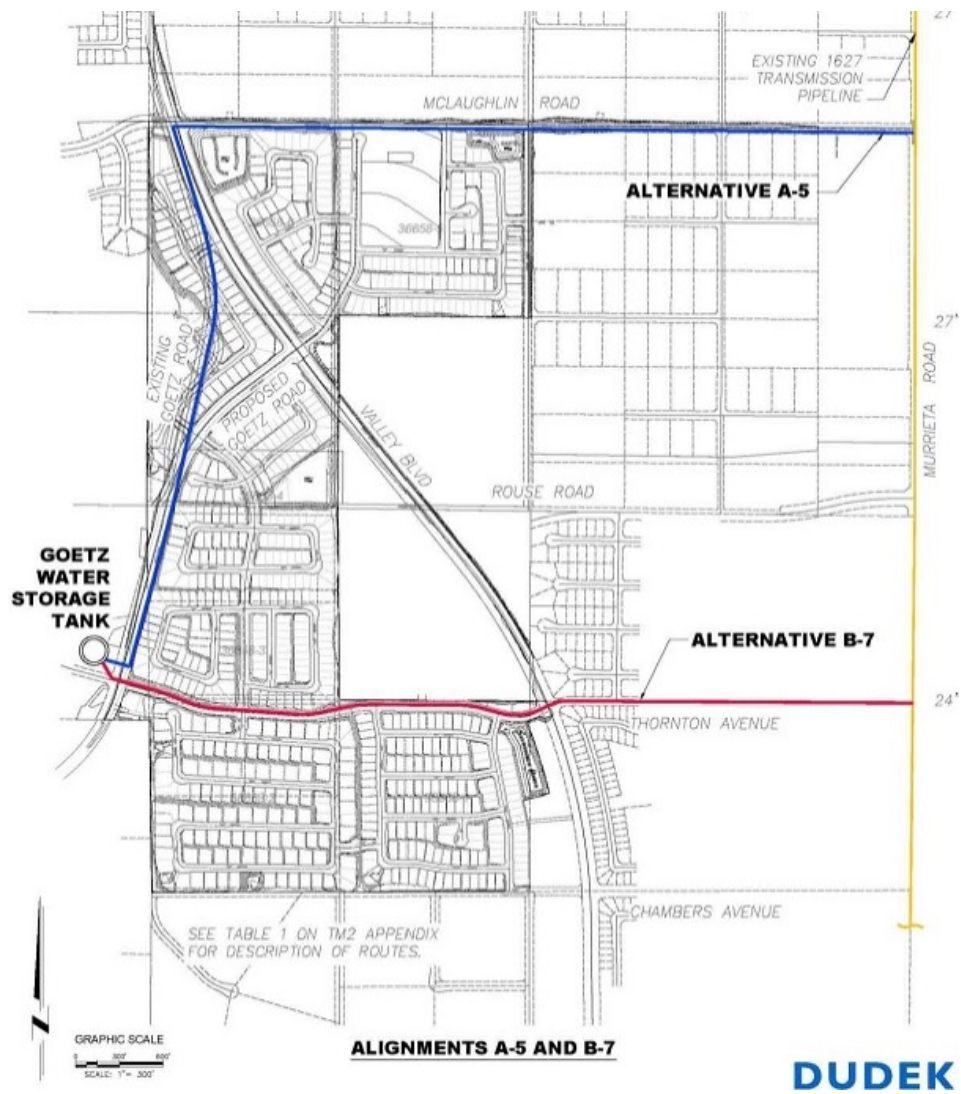
Figure 1 Goetz Road Tank and Transmission Pipeline (B-7 Preferred Alignment)
